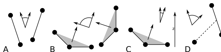
Fig. 5.56: Angle options of gmx gangle (page 182): A. Angle between two vectors. B. Angle between two planes. C. Angle between a vector and the z axis. D. Angle between a vector and the normal of a sphere. Also other combinations are supported: planes and vectors can be used interchangeably.
