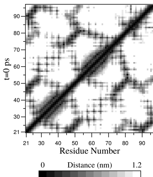
Fig. 5.57: A minimum distance matrix for a peptide 168 (page 575).
