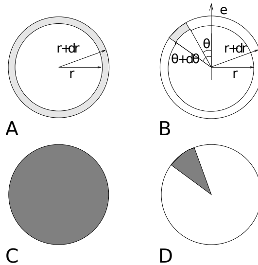
Fig. 5.52: Definition of slices in gmx rdf (page 240): A. g_{AB}(r) . B. g_{AB}(r, \theta) . The slices are colored gray. C. Normalization \langle \rho_B \rangle_{local} . D. Normalization \langle \rho_B \rangle_{local, \theta} . Normalization volumes are colored gray.
